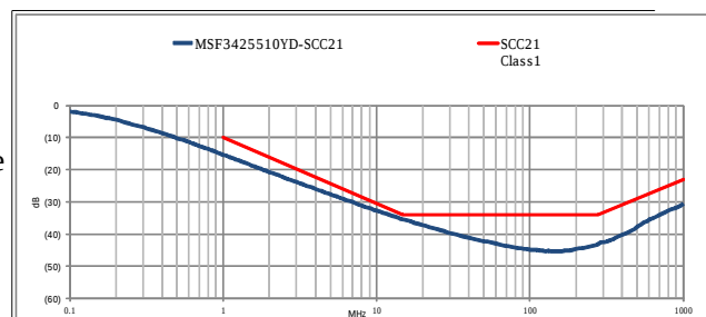
( 2 ) S_{cc21} Curve
