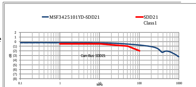
( 1 ) S_{dd21} Curve
