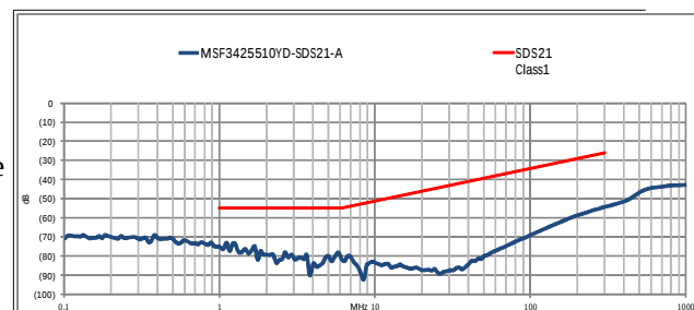
( 3 ) S_{ds21} Curve
